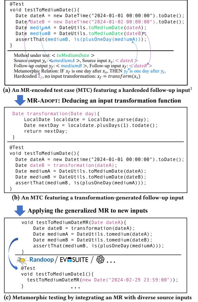
Figure 1: Overview of MR-ADOPT for Metamorphic Testing (i.e., assertions) in MTCs as oracles to verify the generated test pairs. We further employ additional inputs to select the most generalizable input transformation as the result.
